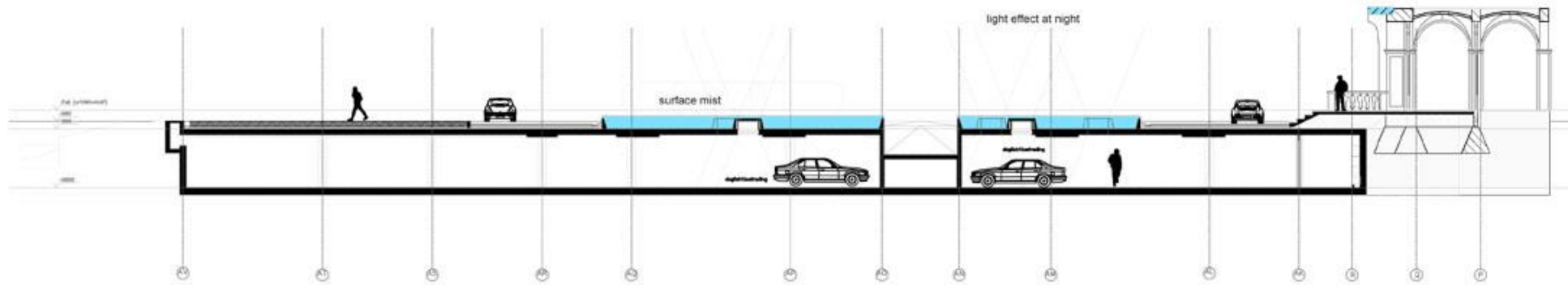
section B-B
